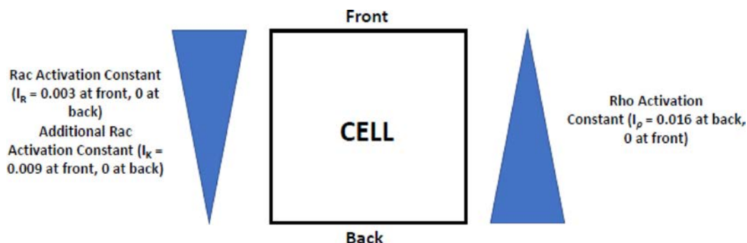
Fig. 4. Schematic showing how the linear gradient in Rac and Rho activation rates is imposed on the 2D domain representing the cell. The range of values for the activation rates are provided in the legends.
